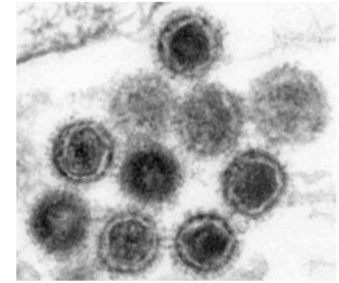
Retrotransposons
