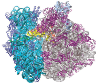
Non-Coding RNAs
